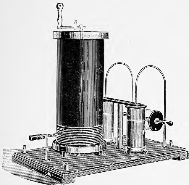
FIG. 35.—SMALL MODEL RESONATOR.
